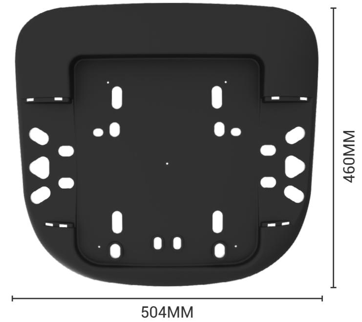
SUPRA SLIMLINE | SHROUD
